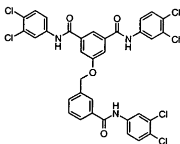
Compound # 38
